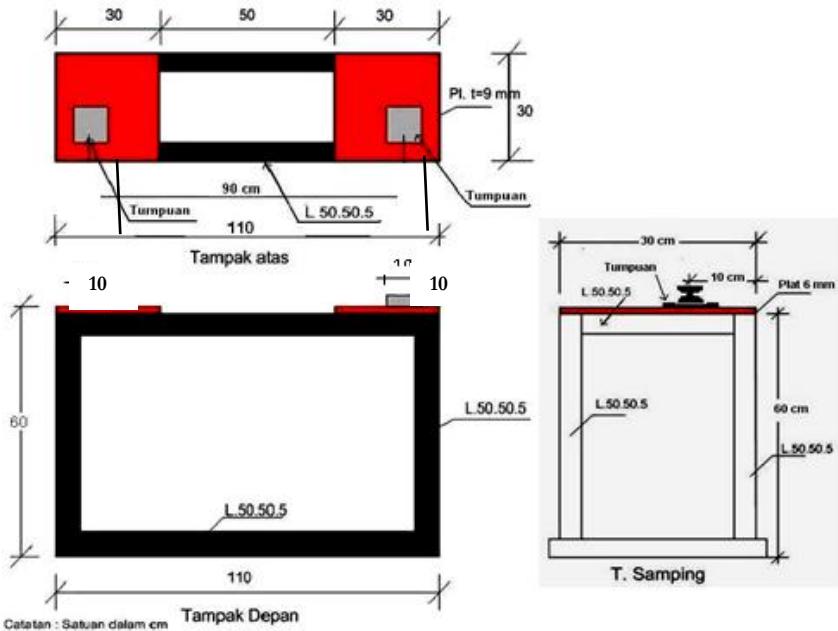
Gambar 5 : GAMBAR ABUTMEN
